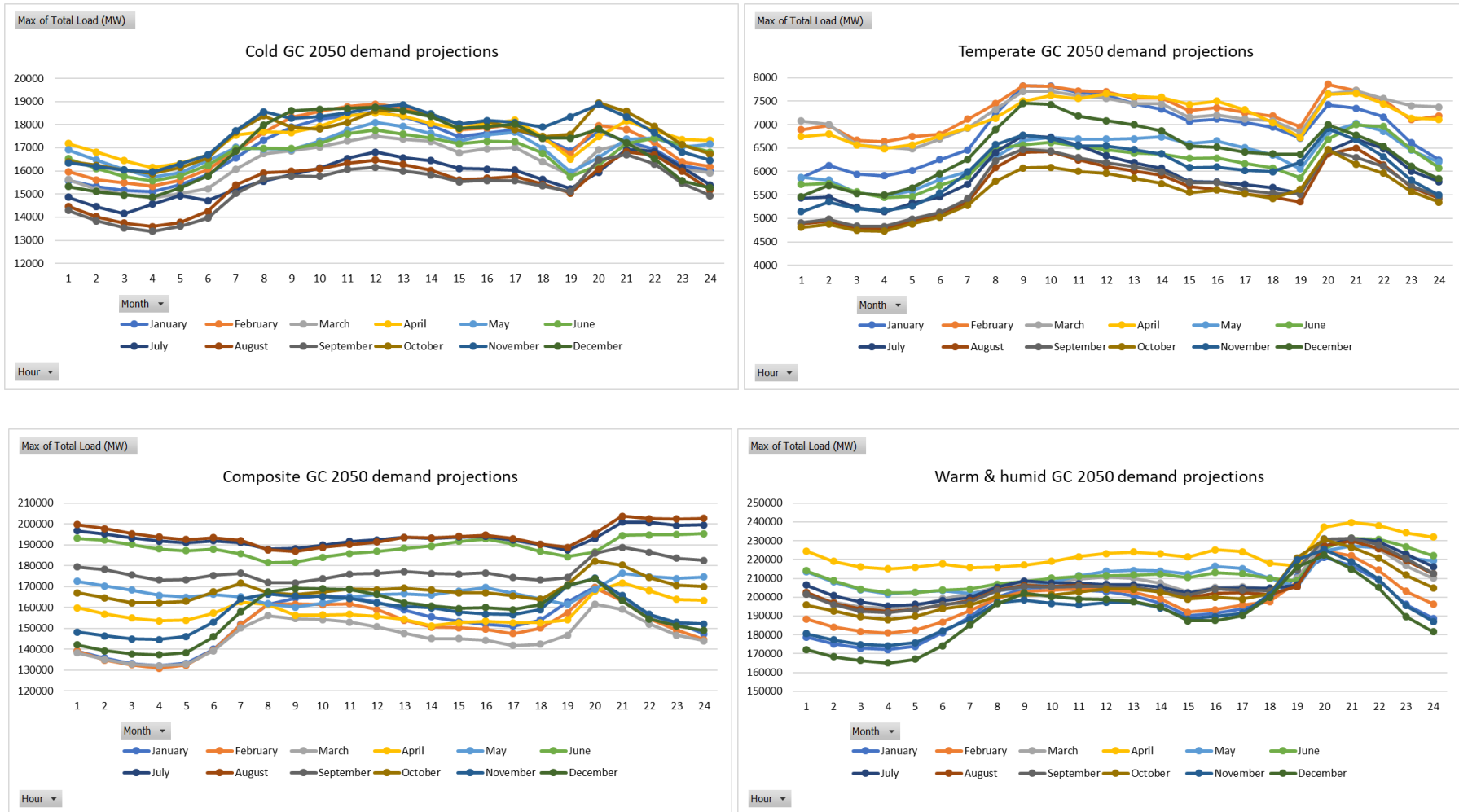
Figure 5. Peak hourly electricity demand profiles for different geo-climatic zones
