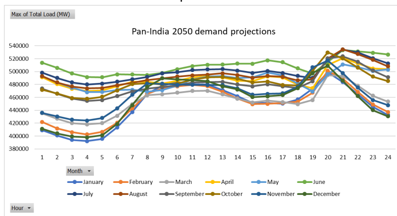
Figure 3. Peak hourly electricity demand profiles at national level
